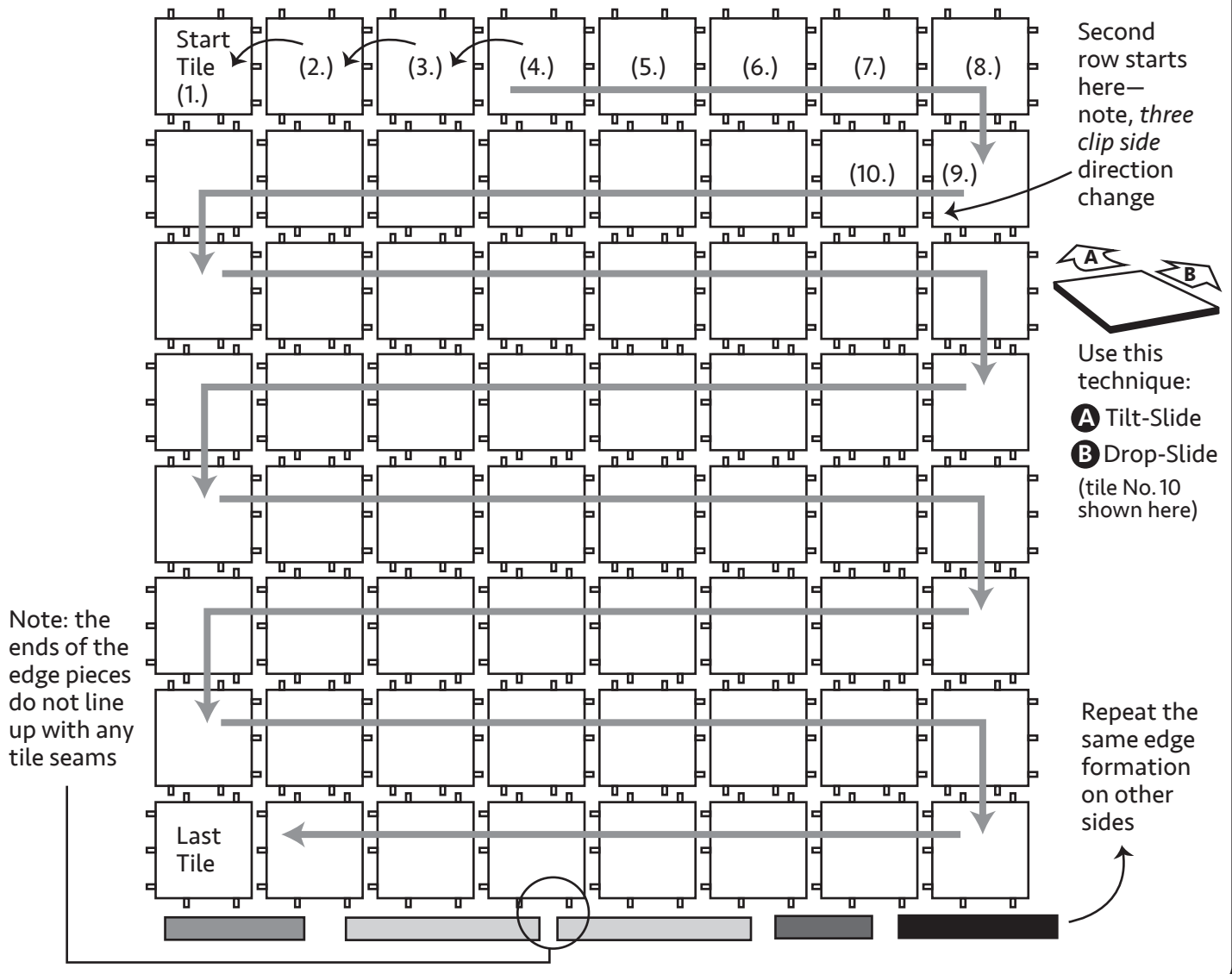
FIGURE A. TILE CONNECTION DIAGRAM (12 x 12 example)
